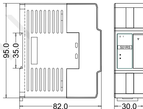
S01RS, H01RS-Dimension figure
