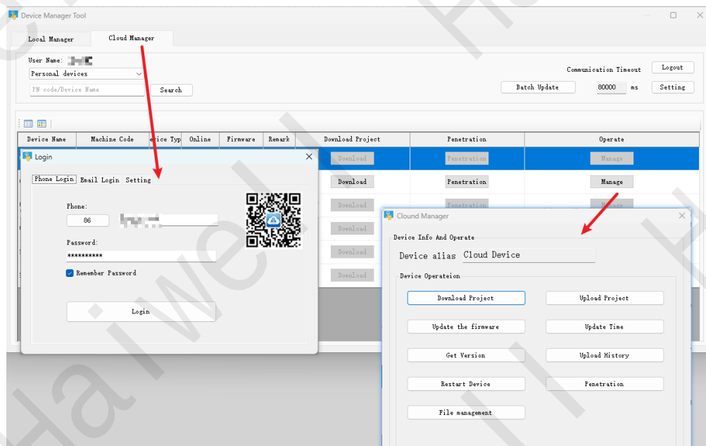
Figure83 Cloud Manager
