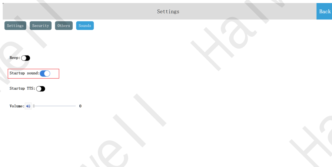
Figure41 Startup Sound
