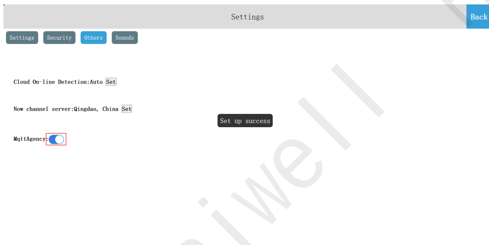
Figure38 MQTT Broker
