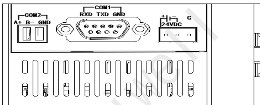
Figure 5 Schematic Diagram of the Bottom Interface of CBOX
