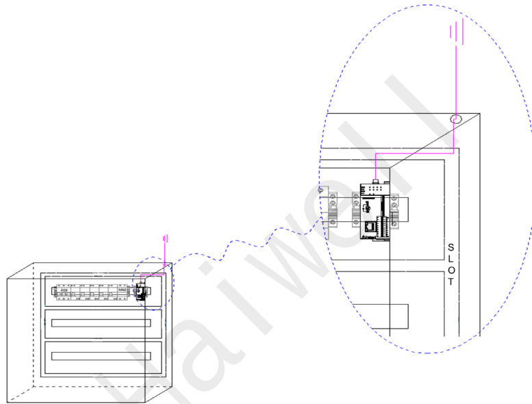
Figure9 Antenna Installation Diagram
