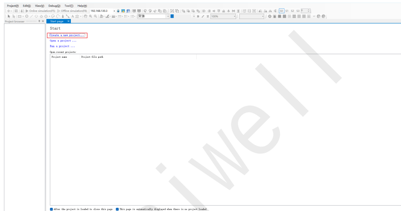
Figure73 New Project
