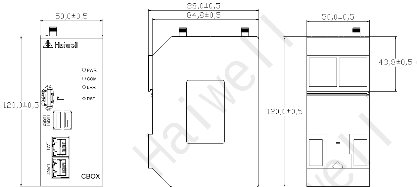
Figure2 Three-view Dimensions of CBOX
