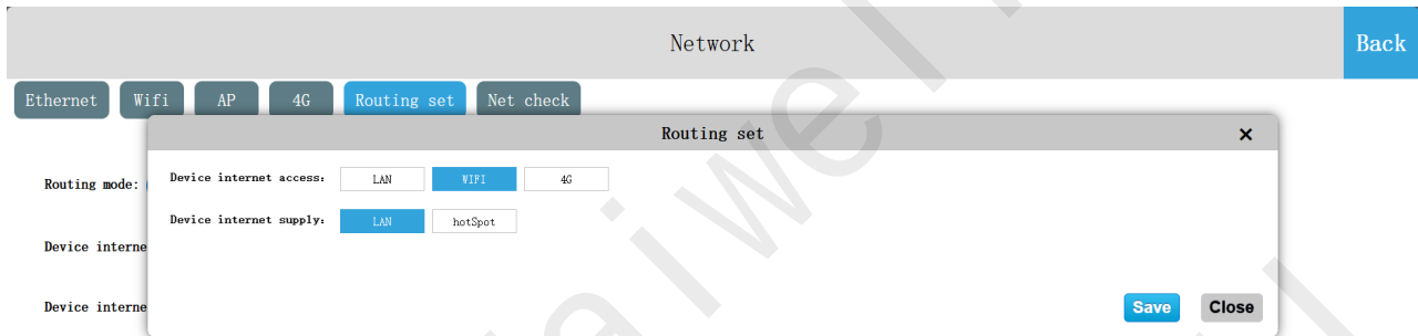
Figure64 Client Mode
