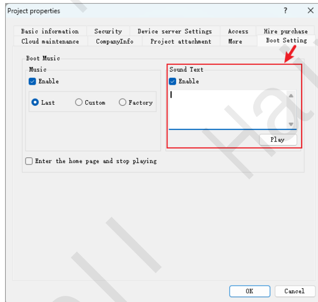
Figure45 TTS Settings
