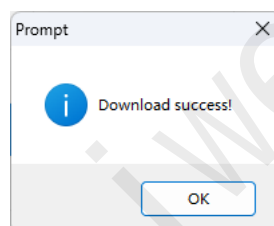
Figure86 Download Successfully
