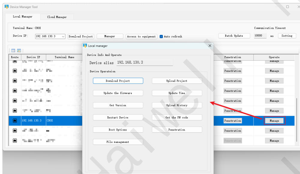
Figure82 Local Manager
