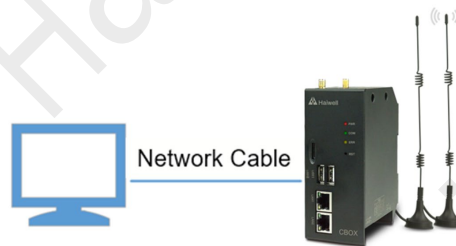
Figure19 Schematic Diagram of CBOX Directly Connected to Computer
