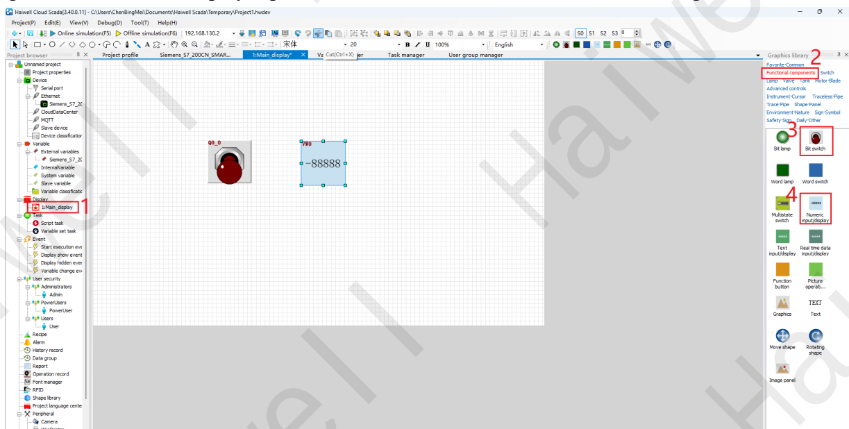
Figure78 Edit Screen
