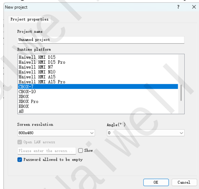
Figure23 Operating Platform
