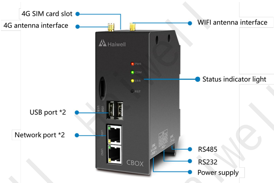
Figure4 Front Interface Diagram of CBOX
