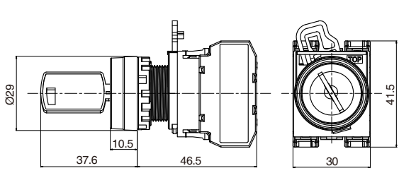
2P钥匙开关 2P Key Switches
