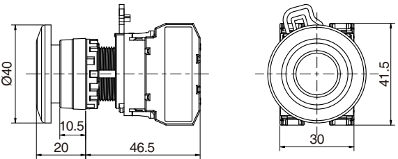
带灯蘑菇头按钮 Illuminated Mushroom head Pushbuttons
