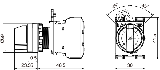
3P带灯选择开关 3P Illuminated Selector Switches
