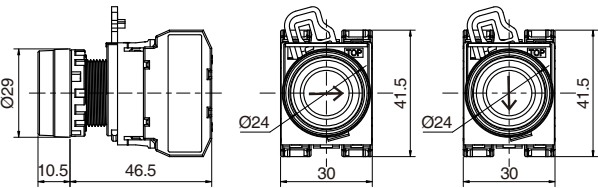
单箭头平头按钮 Single Arrow Flush Pushbuttons
