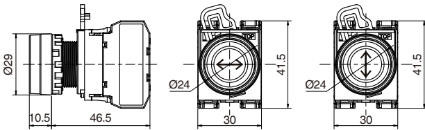
双箭头平头按钮 Double Arrow Flush Pushbuttons
