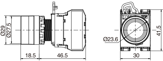
带灯平头按钮 Illuminated Flush Pushbuttons
