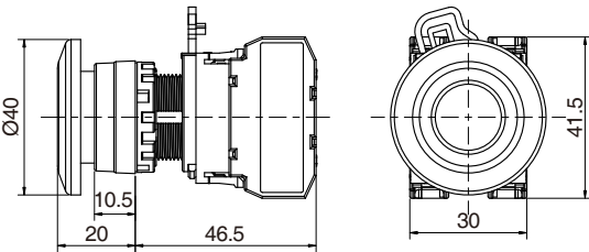
蘑菇头按钮 Mushroom head Pushbuttons
