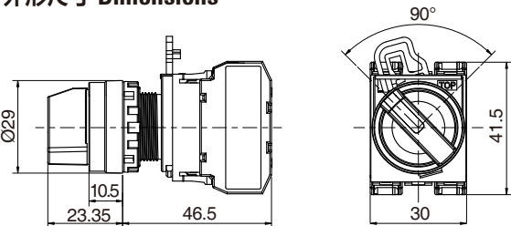
2P选择开关 2P Selector Switches
