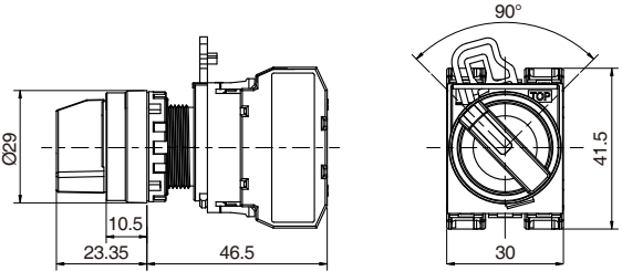
2P带灯选择开关 2P Illuminated Selector Switches
