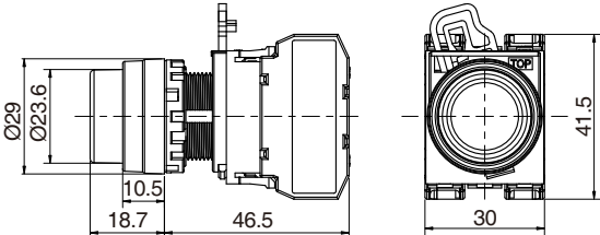
带灯高头按钮 Illuminated Extended Pushbuttons
